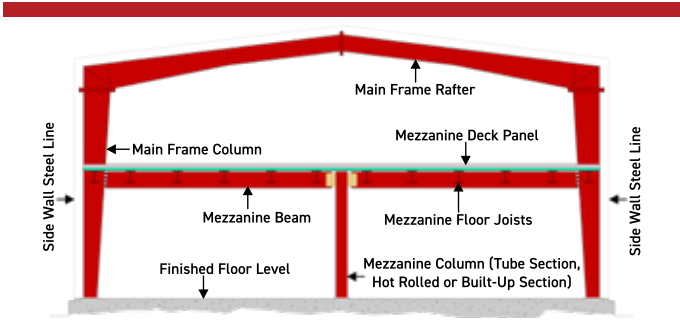
Primary Framing
